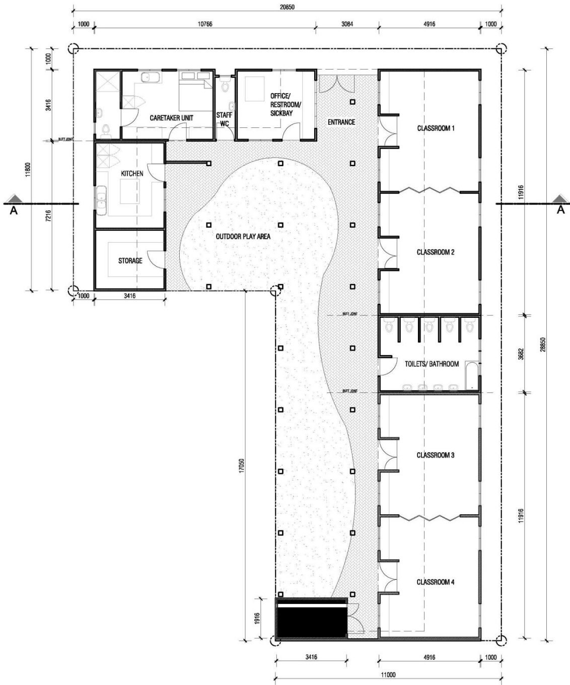
PLAN LAYOUT 1:100
